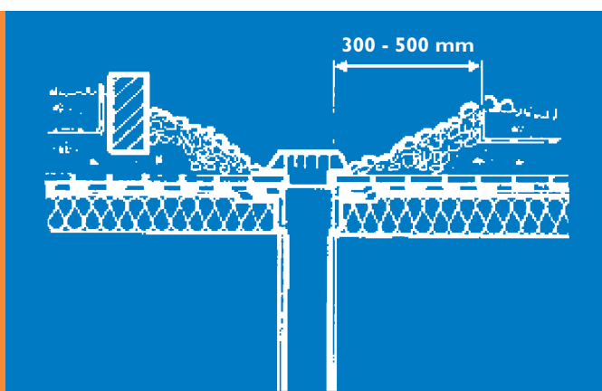
Fig. 9 – Gravel Skirt and Vegetation Barrier Around Roof Drain
