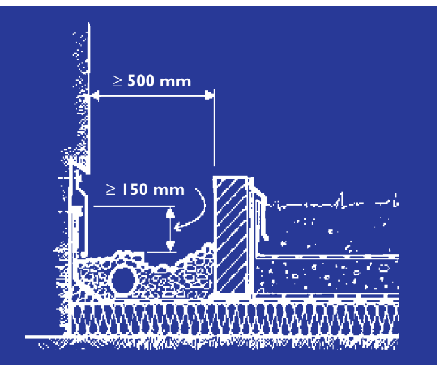
Fig. 10 – Flashing and Gravel Barrier with Drainage Pipe at a Wall/Roof Connection
