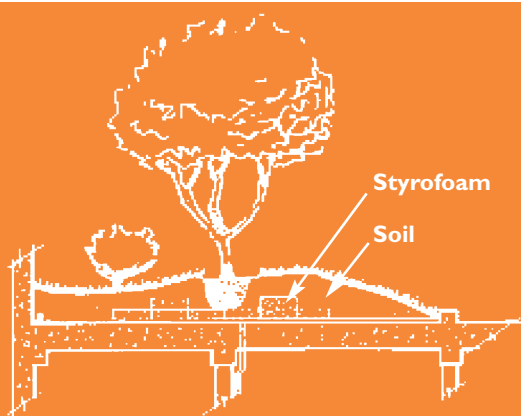
Fig. 8 – Deep Soil over Structural Column
